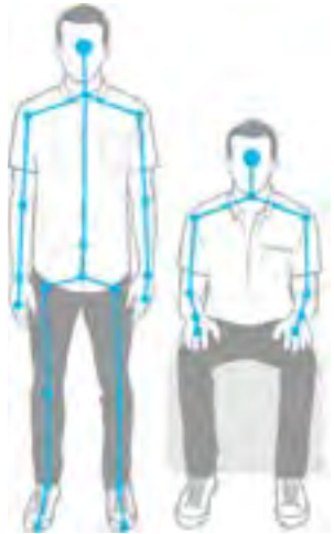
Skeleton Tracking
